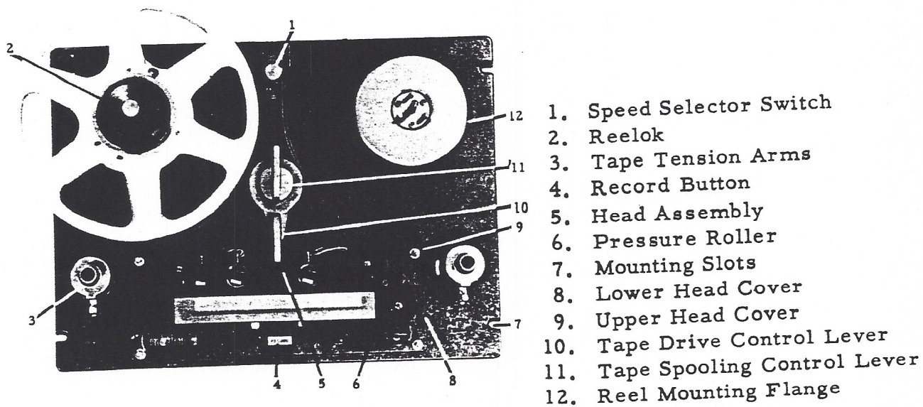
Fig. 1 DRIVE PANEL, FRONT VIEW (HEAD COVERS GHOSTED)
