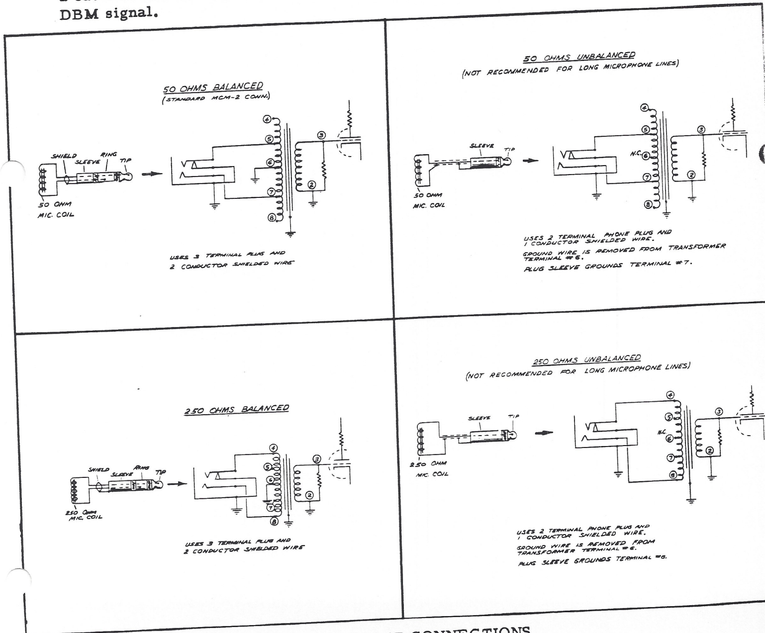
Fig. 4 INPUT CONNECTIONS
